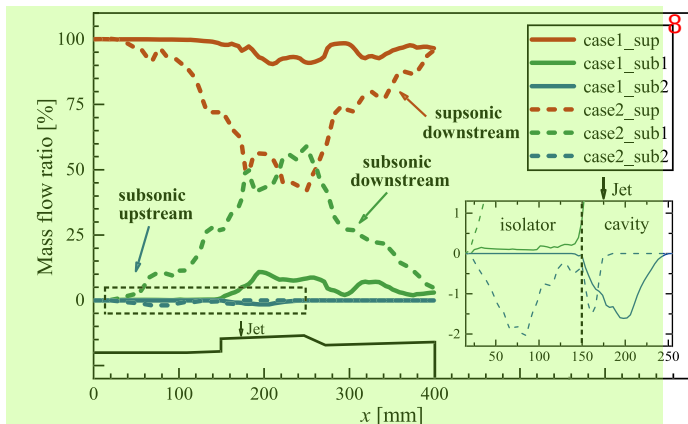
Fig. 9. Time-averaged mass flow ratio of combined speed and direction.
