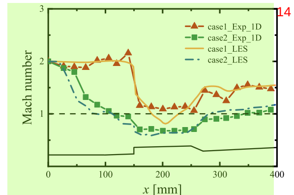
Fig. 4. Experimental and computational 1-D Mach number distribution
