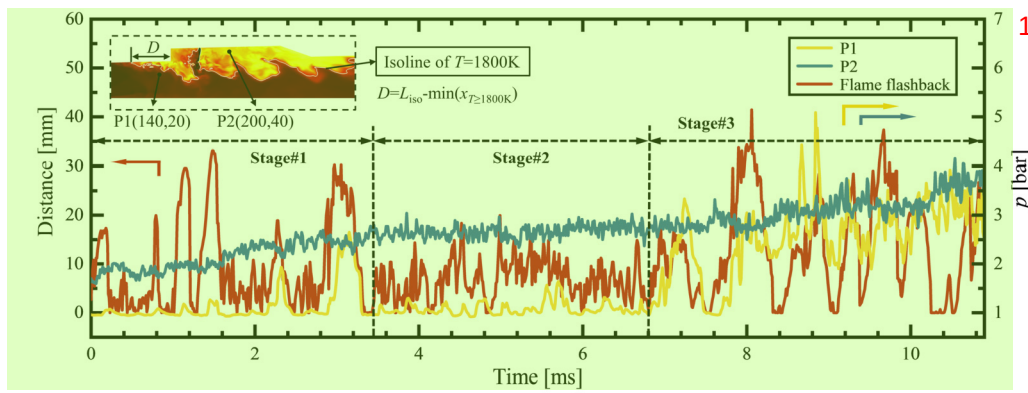
Fig. 12. Temporal histories of pressure signal and flame flashback distance oscillation.
