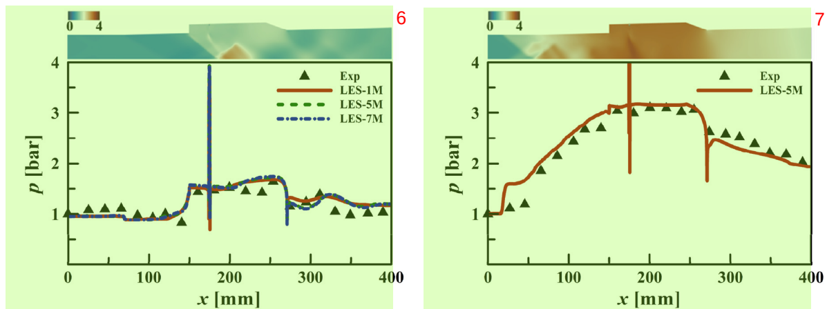
Fig. 3. Comparison of computational pressure profiles on the upper wall of case 1 (left) and case 2 (right) with Tian's experimental results
